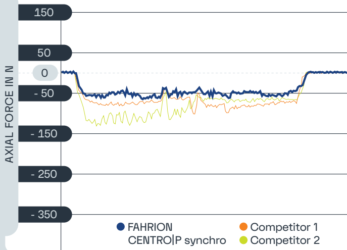
Force measurement during thread forming of M6 without IC
