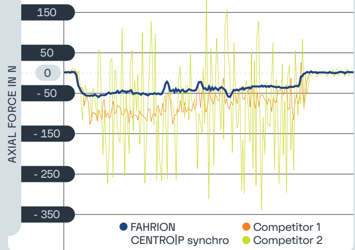
Force measurement during thread forming of M6 with IC
